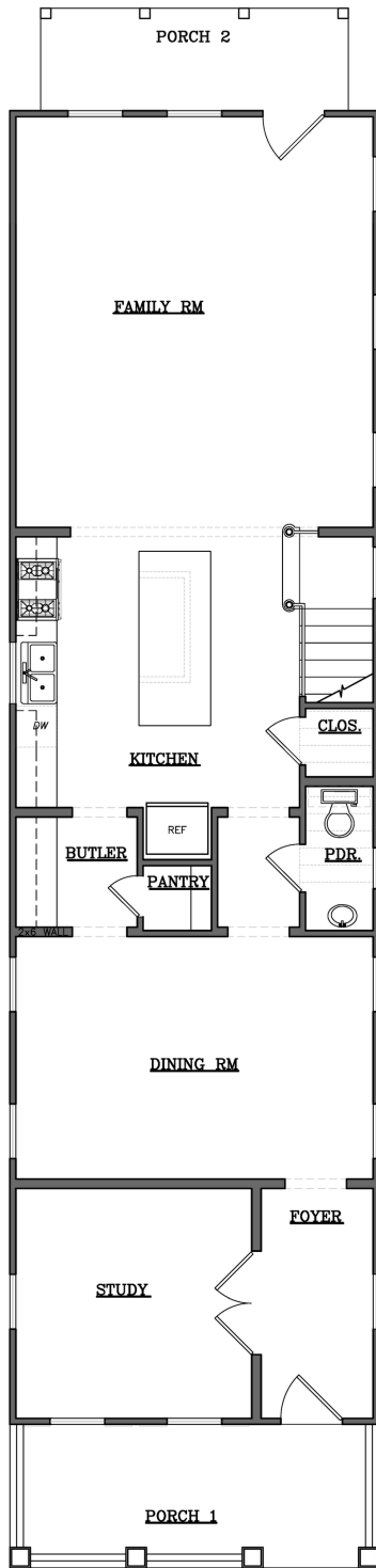
FIRST FLOOR
